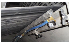
A Model 110048PKI 48" (1219mm) Super Air Knife with Plumbing Kit installed uses EXAIR's Universal Air Knife Mounting System to maintain proper position for removing dust on a conveyor belt and eliminate carryover accumulation.
