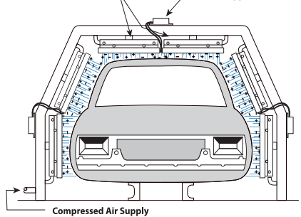
(6) Model 112024 24" (610mm) Gen4 Super Ion Air Knives (3) Model 7960 Gen4 Power Supplies
